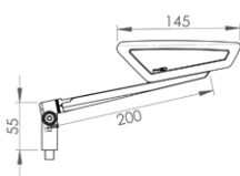
ADAPTABLE Avaible adapters for handlebar and fairing fitting.
