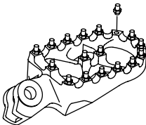
DESIGN Maximum grip with replaceable tips.
