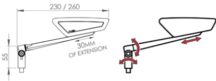
ADJUSTABLE Inclination, adjustment, and extension of the mirror.
