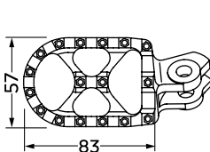
DIMENSIONS 83 x 57 mm.
