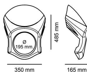
CV8 VARIANT 2 PART#9553/9515
