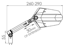
ADJUSTABLE Inclination, adjustment, and extension of the mirror.
