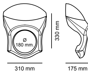
CV7 VARIANT 2 PART# 9554/9516
